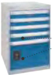
4-DRAWER W/ONE DOOR CABINETS Model FH670 (4) 15 3/8" W x 20" D x 2 5/8" H (1) 16 3/4" W x 21" D x 12" H Weight: 63 lbs.
